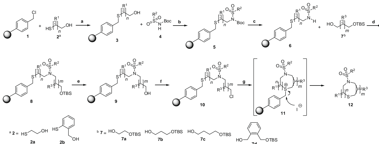
Scheme 2. Reagents and conditions: (a) 2 (3 equiv), DBU (4 equiv), DMF, rt, 24 h; (b) 4 (4 equiv), PPh 3 (4 equiv), DEAD (4 equiv), THF, rt, 24 h; (c) n -BuNH 2 , rt, 24 h; (d) 7 (4 equiv), TMAD (4 equiv), n -Bu 3 P (4 equiv), THF, rt, 24 h; (e) 1 M TBAF/THF, rt, 24 h; (f) Cl 3 CCl 3 (4 equiv), PPh 3 (4 equiv), CH 2 Cl 2 , rt, 24 h; (g) CsI (2 equiv), piperidinomethyl polystyrene (2 equiv), dioxane, water, 180 °C, 1–2 h.
